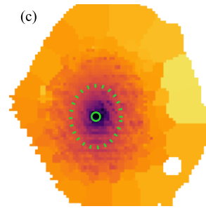
\log \Sigma_{\star}^{\text{dez}} [ M_{\odot} \text{pc}^{-2} ]
