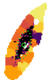
\sigma_{\star} [\text{km s}^{-1}]
