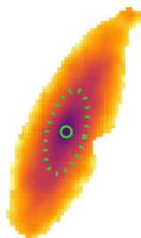
\langle \log Z \rangle_M [Z_{\odot}]
