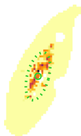
\log \Sigma_{\text{SFR}} [M_{\odot} \text{Gyr}^{-1} \text{pc}^{-2}]
