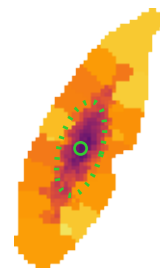
\log \Sigma_{\star}^{\text{dez}} [M_{\odot} \text{pc}^{-2}]
