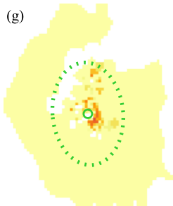
\log \Sigma_{\text{SFR}} [ M_{\odot} \text{ Gyr}^{-1} \text{ pc}^{-2} ]
