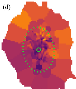
\langle \log t \rangle_L [yr]
