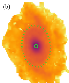
\log \mathcal{L}_{5635\text{\AA}} [ L_{\odot} \text{ pc}^{-2} ]
