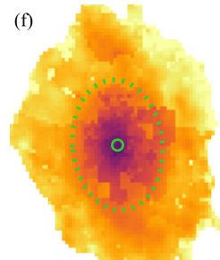
\log \Sigma_{\star}^{\text{dez}} [ M_{\odot} \text{ pc}^{-2} ]
