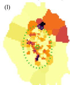
\sigma_{\star} [ \text{km s}^{-1} ]
