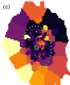
\langle \log Z \rangle_M [ Z_{\odot} ]
