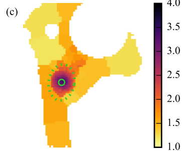
\log \Sigma_{\star}^{\text{dez}} [M_{\odot} \text{pc}^{-2}]
