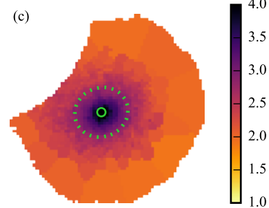
\log \Sigma_{\star}^{\text{dez}} [M_{\odot} \text{pc}^{-2}]
