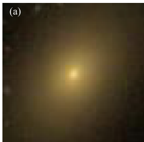
SDSS image
