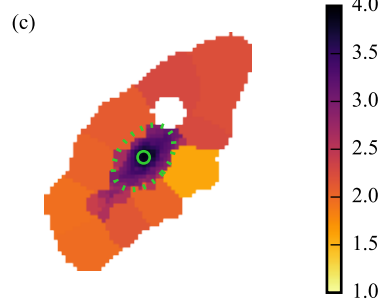
\log \Sigma_{\star}^{\text{dex}} [\text{M}_{\odot} \text{pc}^{-2}]
