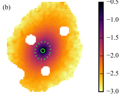
\langle \log Z \rangle_{\text{M}} [Z_{\odot}]
