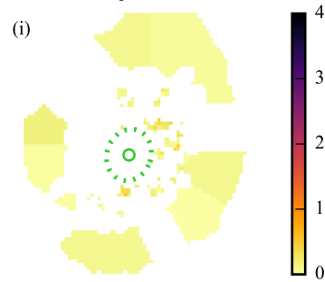
\sigma_{\star} [\text{km s}^{-1}]
