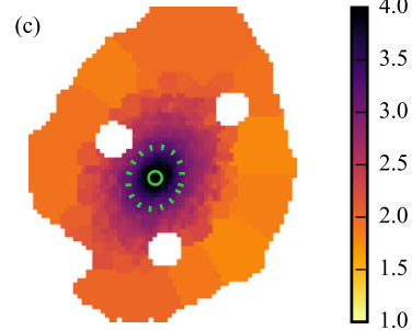
\log \Sigma_{\star}^{\text{dez}} [\text{M}_{\odot} \text{pc}^{-2}]
