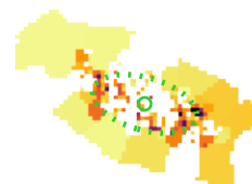
\sigma_{\star} [\text{km s}^{-1}]
