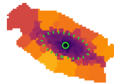
\log \Sigma_{\star}^{\text{dez}} [M_{\odot} \text{pc}^{-2}]
