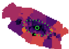
\log \Sigma_{\text{SFR}} [M_{\odot} \text{Gyr}^{-1} \text{pc}^{-2}]
