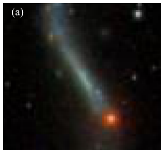
SDSS image
