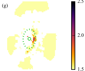
\log \Sigma_{\text{SFR}} [M_{\odot} \text{Gyr}^{-1} \text{pc}^{-2}]
