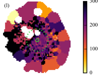
\sigma_{\star} [\text{km s}^{-1}]
