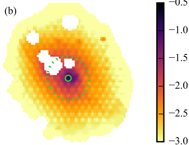
\langle \log Z \rangle_{\text{M}} [Z_{\odot}]
