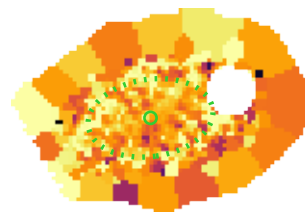
\sigma_{\star} [ \text{km s}^{-1} ]
