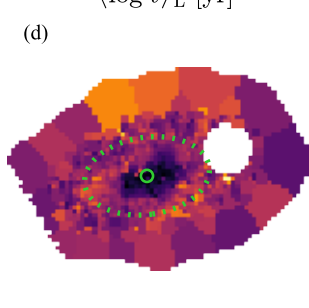
\log \Sigma_{\text{SFR}} [ M_{\odot} \text{Gyr}^{-1} \text{pc}^{-2} ]
