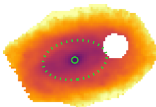
\langle \log Z \rangle_M [ Z_{\odot} ]
