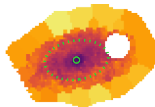
\log \Sigma_{\star}^{\text{dez}} [ M_{\odot} \text{pc}^{-2} ]
