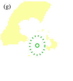
\log \Sigma_{\text{SFR}} [M_{\odot} \text{Gyr}^{-1} \text{pc}^{-2}]
