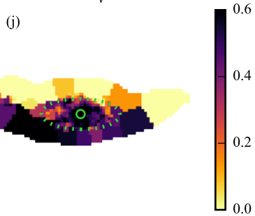
\tau_V
