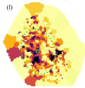
\sigma_{\star} [\text{km s}^{-1}]
