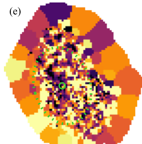
\langle \log Z \rangle_{\text{M}} [Z_{\odot}]
