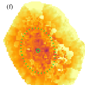
\log \Sigma_{\star}^{\text{dez}} [\text{M}_{\odot} \text{pc}^{-2}]
