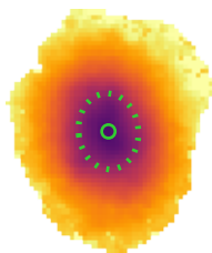
\langle \log Z \rangle_M [\text{Z}_{\odot}]
