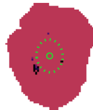
\sigma_{\star} [\text{km s}^{-1}]
