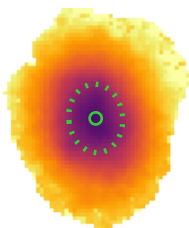
\langle \log Z \rangle_M [\text{Z}_{\odot}]
