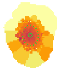
\log \Sigma_{\star}^{\text{dez}} [\text{M}_{\odot} \text{pc}^{-2}]
