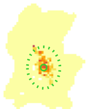
\log \Sigma_{\text{SFR}} [M_{\odot} \text{Gyr}^{-1} \text{pc}^{-2}]
