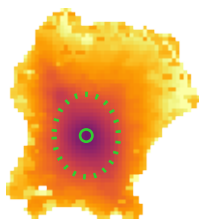
\log \mathcal{L}_{5635\text{\AA}} [L_{\odot} \text{pc}^{-2}]
