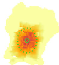
\log \Sigma_{\star}^{\text{dez}} [M_{\odot} \text{pc}^{-2}]
