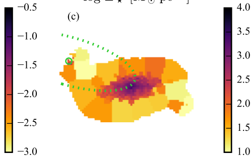
\log \Sigma_{\star}^{\text{dez}} [ M_{\odot} \text{pc}^{-2} ]
