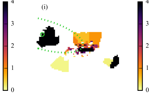
\sigma_{\star} [ \text{km s}^{-1} ]
