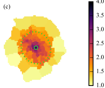
\log \Sigma_{\star}^{\text{dez}} [M_{\odot} \text{pc}^{-2}]
