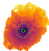
\log \Sigma_{\star}^{\text{dez}} [M_{\odot} \text{pc}^{-2}]
