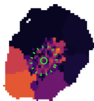
\langle \log Z \rangle_M [Z_{\odot}]
