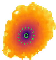
\log \mathcal{L}_{5635\text{\AA}} [L_{\odot} \text{pc}^{-2}]
